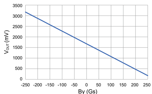
TMR2625D-AAI Y-axis output curve
