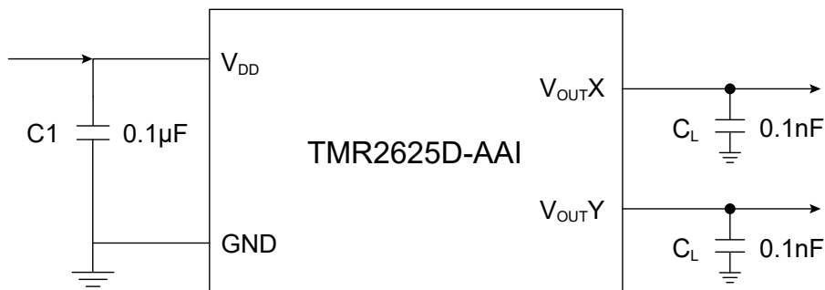
Figure 7. Application circuit diagram
