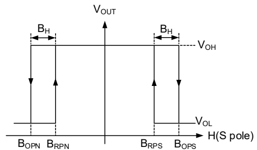
Figure 4. Switching characteristics
