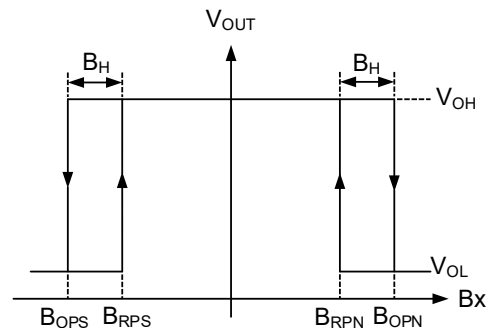
Figure 3. Switching characteristics
